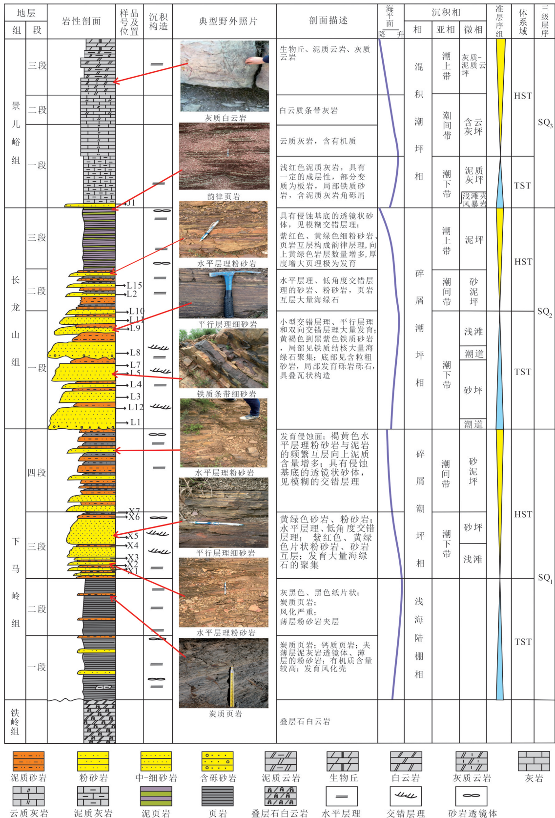
Fig. 2 Comprehensive column chart showing the sequence stratigraphy and sedimentary facies of the Qingbaikouan System, Longshan area, North China
